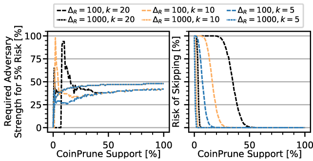
Fig. 4. Larger reconfirmation windows increase CoinPrune’s resilience against adversaries independent from the acceptance threshold.
